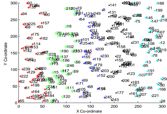
Fig 9: Second level hierarchical formation with differentiated colours indicating difference in five clusters. Using MATLAB, all 250 nodes were randomly distributed as shown in Fig. 5 with the BS whose location is (150,150) was situated. With the initial energy level of all nodes being set at 200 J, E_{elec} set to 50 nJ/bit, E_{amp} set to 100 pJ/bit/m 2 , and the size of the sensor data set to 1024 bits, we used the radio model equation to evaluate residual energy level for cluster head selection, data aggregation and transmission phase for 400 rounds for non hierarchical formation scenario, first level hierarchical formation scenario and second level hierarchical formation scenario. The cluster head(s) of m -th cluster formed aggregates the data received from other sensor nodes with its own data and transmits it to the next hop cluster head closer to the base station or to the base station depending on the cluster formation and the shortest distance between the cluster head and the BS. At every transmission or reception made, energy reduction occurs for every node, thereby cluster head rotation was utilized to help prolong the lifetime of the WSN.
